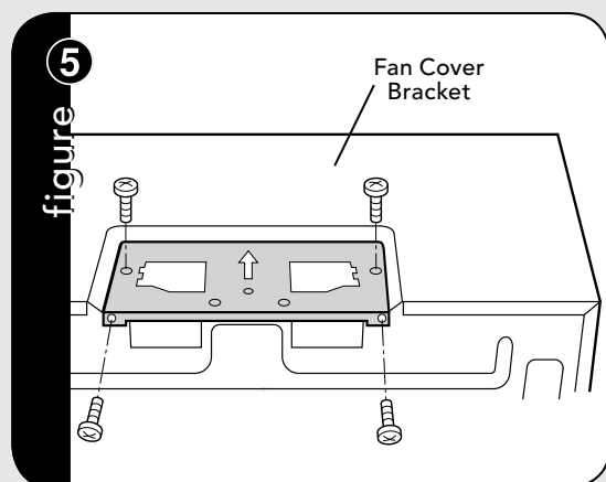
HORIZONTAL EXHAUST: Remove and save 4 screws. Remove fan cover bracket.
