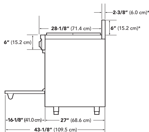
VGRC485-4GD Four-Burner/ Double Griddle Range
